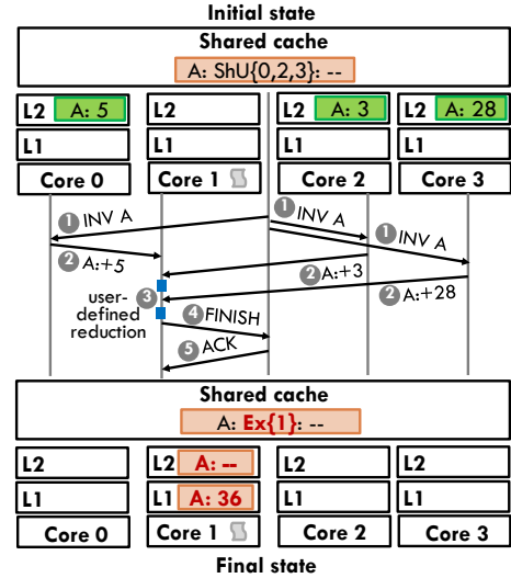
Fig. 7. Reductions are triggered by non-commutative requests. In this example, core 1 issues an unlabeled or differently-labeled request, causing a full reduction of line A’s U-state data, held in several private caches.
